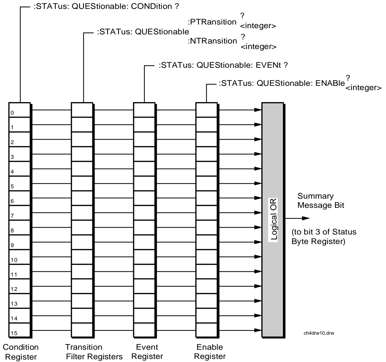
Figure 27 Questionable Data/Signal Register Group
