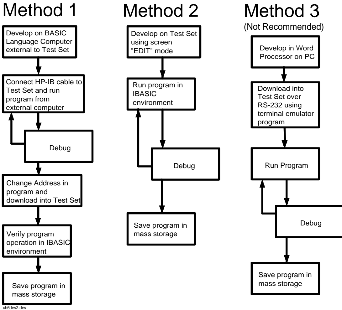
Figure 38 Program Development Methods
