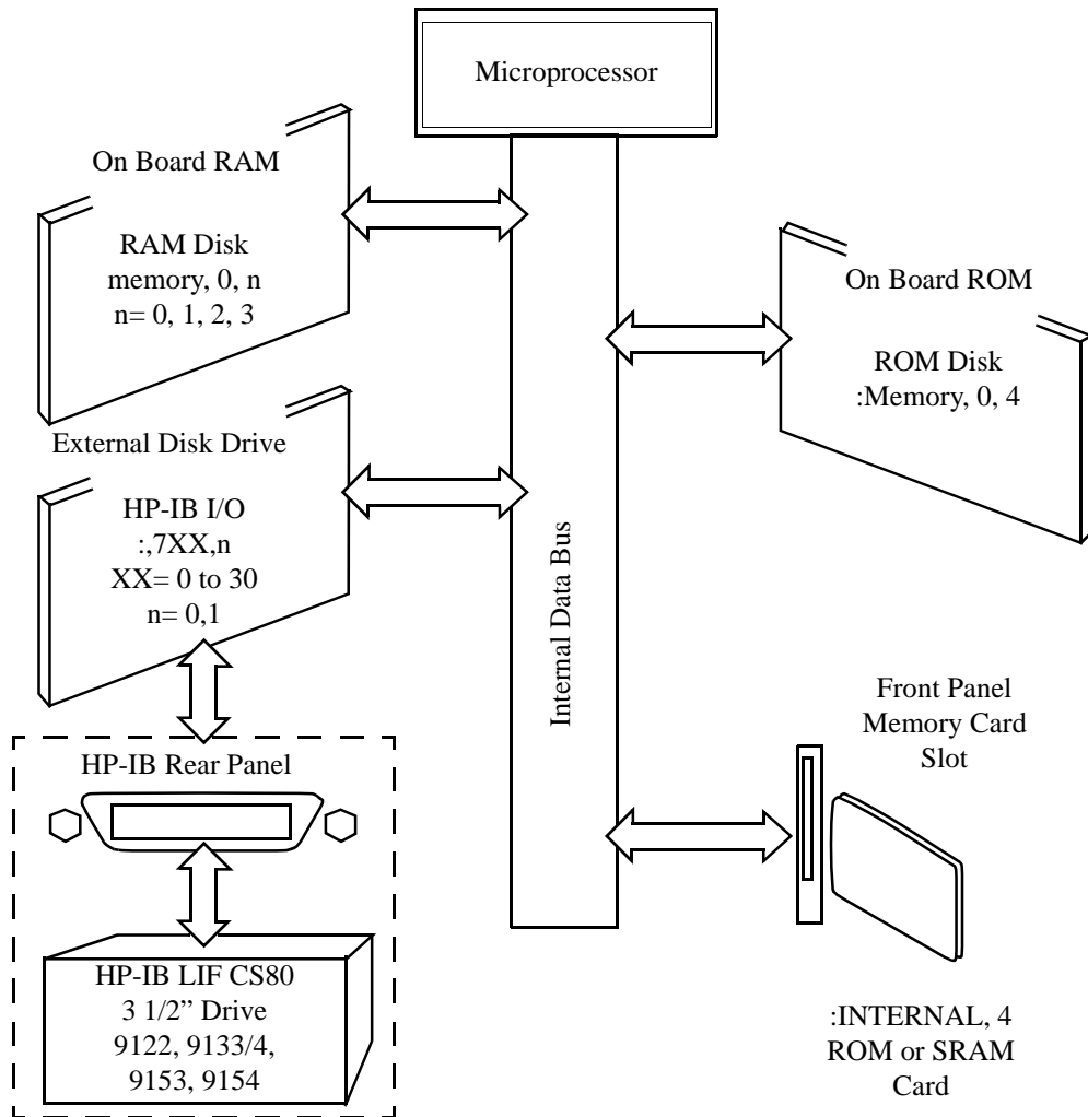
Figure 33 Internal and External Mass Storage Devices
