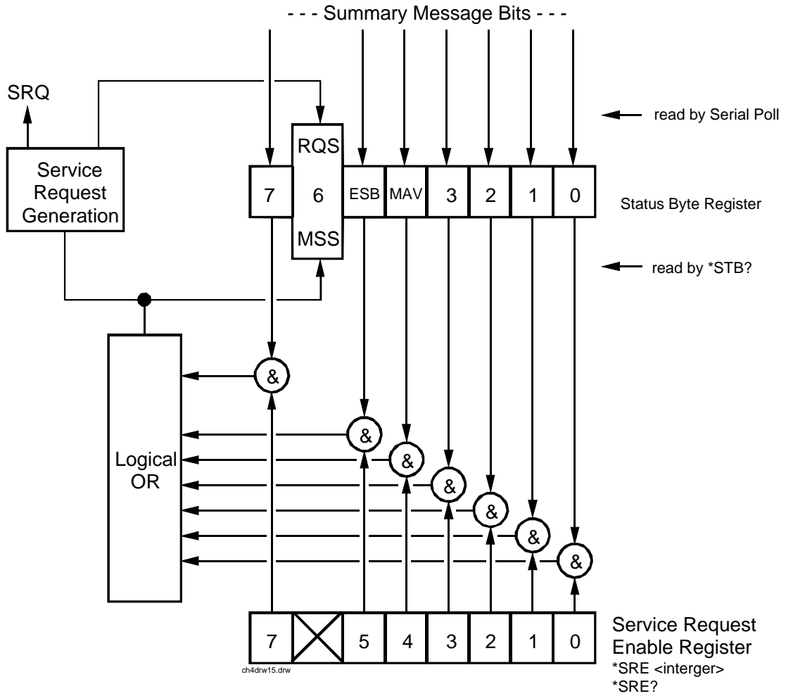
Figure 31 Status Byte/Service Request Enable Register
