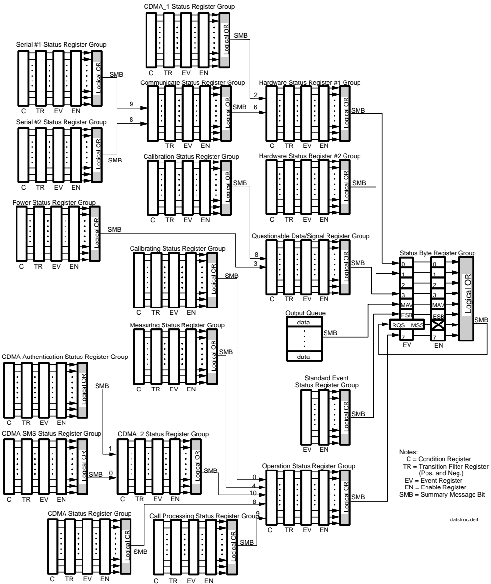
Figure 10 Test Set Data Structure Block Diagram
