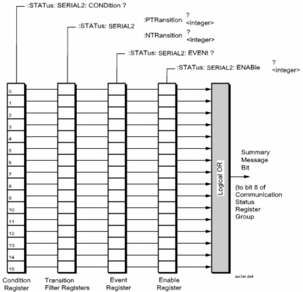
Figure 29 Serial 2 Status Register Group
